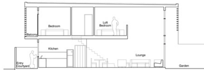
Long Section
