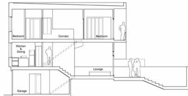
Long Section
