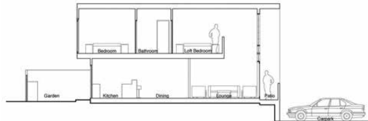
Long Section
