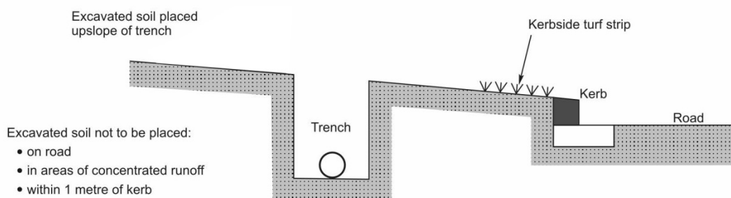
Figure 111: Typical trenching methodology
