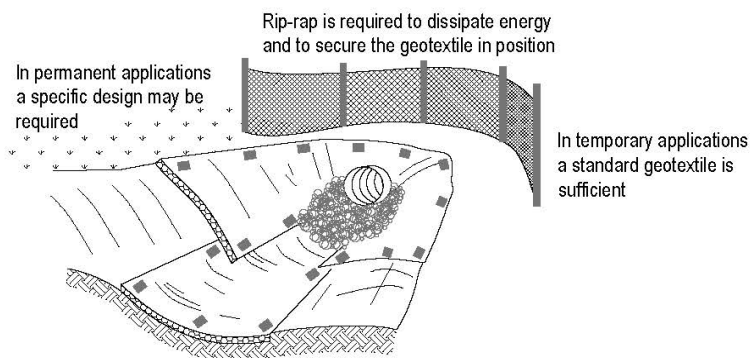
Figure 60: Geotextile design – on slopes
