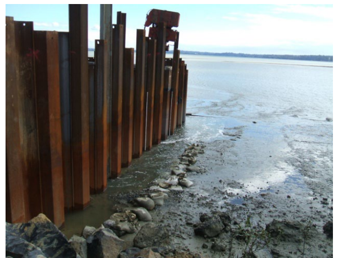
Figure 133: Water draining from a sheet pile coffer dam
