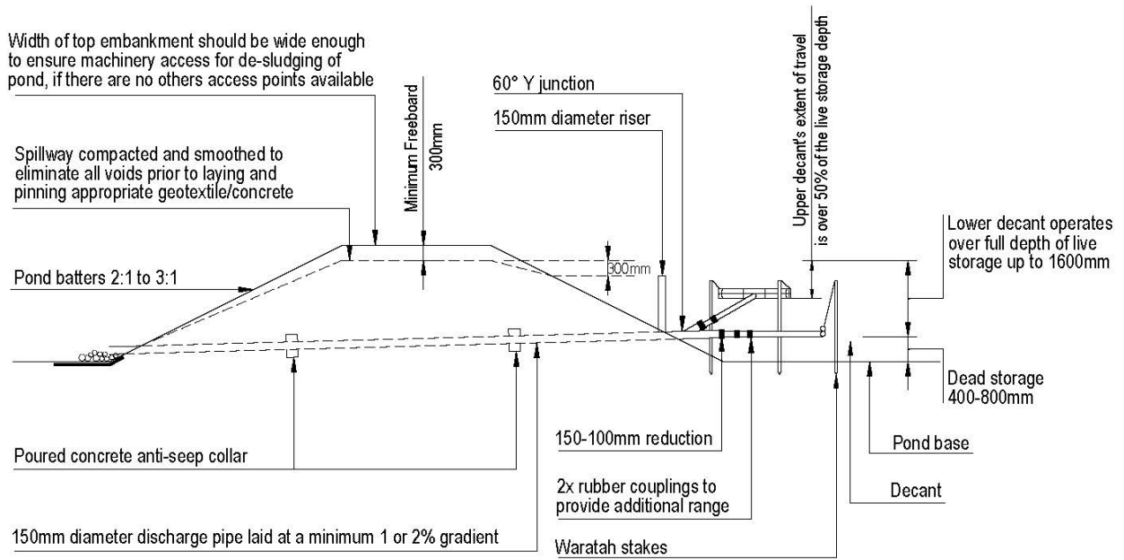
Cross - section
