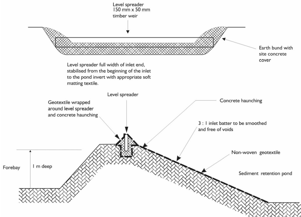
Figure 70: Level spreader
