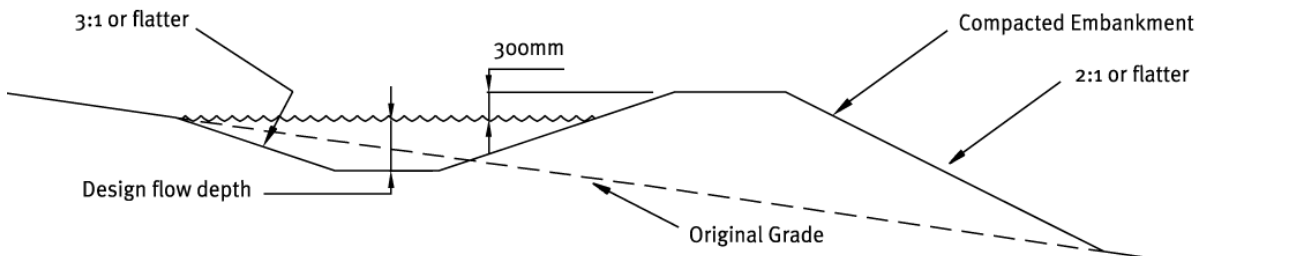
Cross Section
