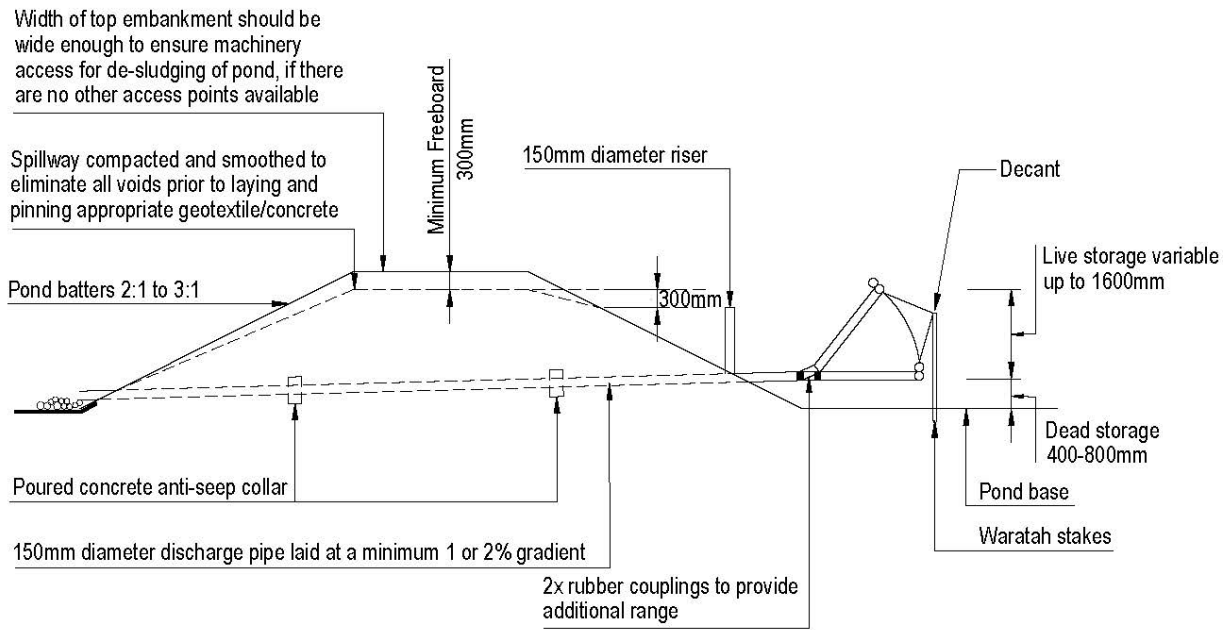
Cross - section
