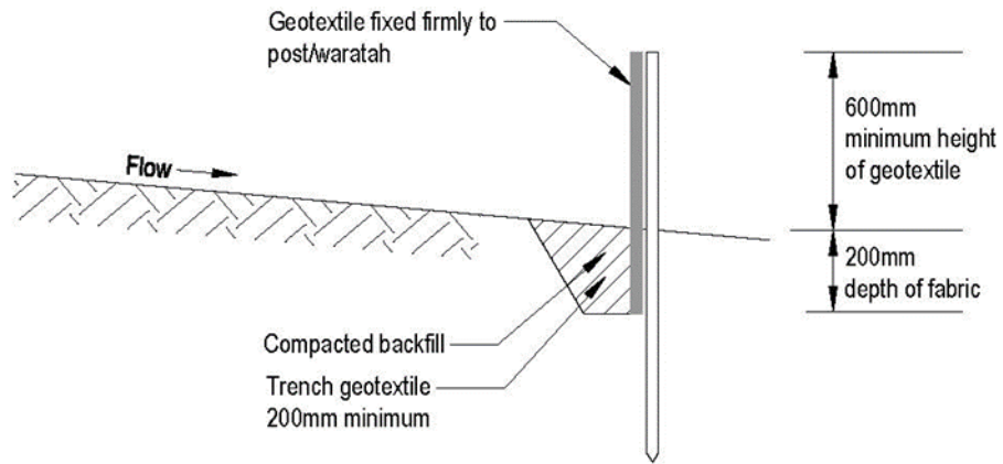
Cross-section
