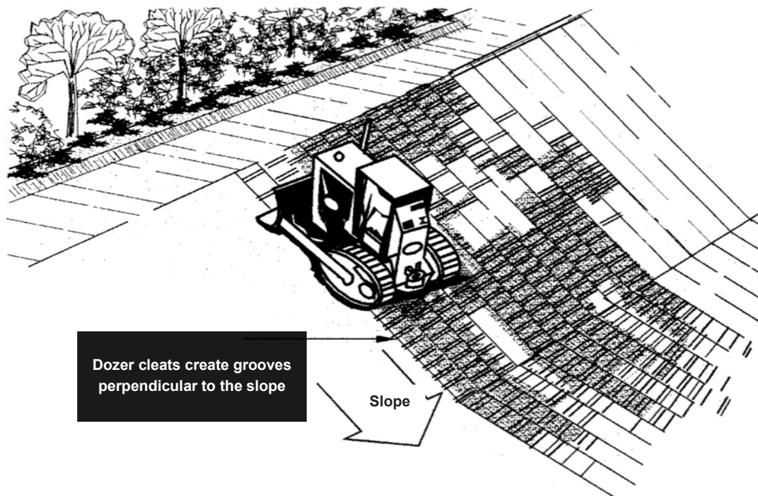
Figure 41: Surface roughening
